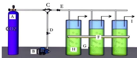
Figure 1. Experimental Setup. Where; A. CO 2 gas tube, B. Air blower, C. Gas mixing point, D. Valve, E. Gas flowmeter, F. Tube Light lamp, G. Photobioreactor, H. Stone aerator, I. Output gas.
